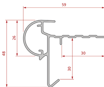
Roval-Round PLUS 147615
